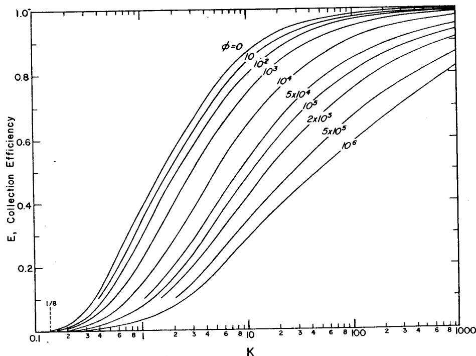
Figure 4. Collection efficiency E is determined by an inertia parameter K and the parameter \Phi
