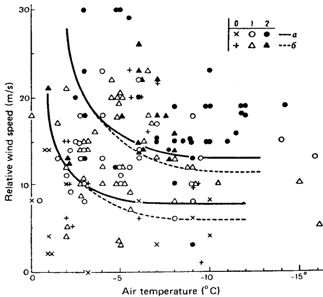
Figure 12. Icing severity as related to air temperature and wind velocity (Borisenkov and Panov 1972, taken from Japanese data in Tabata et al. 1963) where a = 450-ton displacement ship; b = 350-ton displacement ship; 0 = no icing; 1 = significant icing; 2 = heavy icing.
