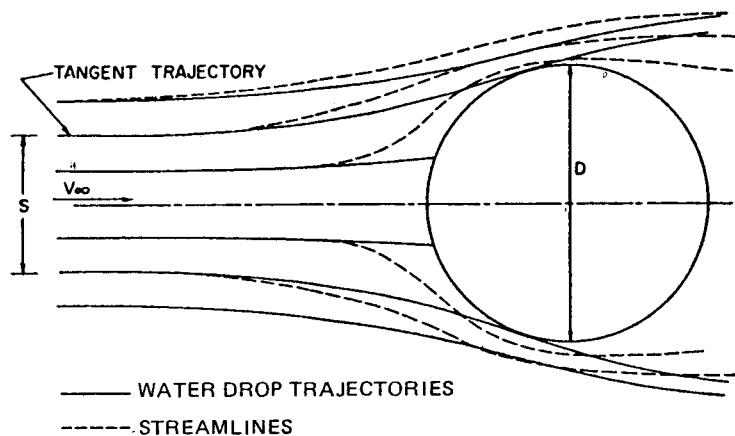
Figure 3. Collection efficiency of a cylinder. Water droplets following trajectories off the center line approach will be deflected and, at a certain distance from the axis, will not impinge on the cylinder. Collection efficiency is the ratio of the mass of droplets striking the cylinder to the total mass that would impinge if they were not deflected. If a constant mass flux is assumed, this can be represented in terms of the linear measures S and D , so that E = S/D (Stallabrass and Hearty 1967).
