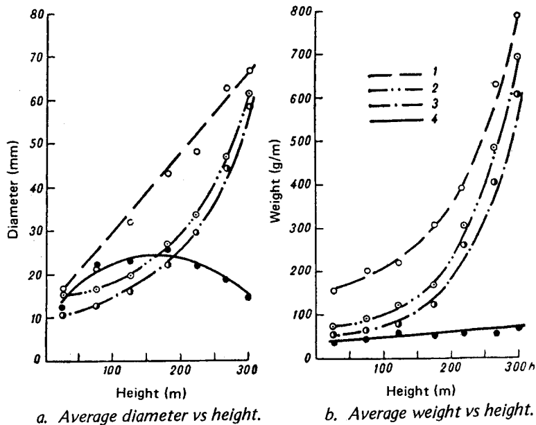
Figure 9. Variation of average diameter and weight of ice accumulation (1—mixture, 2—hard rime, 3—glaze ice, 4—soft rime) with height on meteorological tower at Obninsk, U.S.S.R. (Glukhov 1972).
