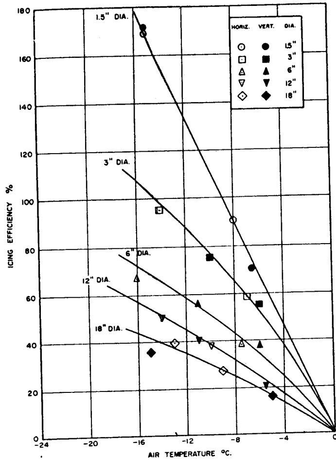
Figure 7. Icing efficiency, i.e. the fraction of water droplets that could strike a cylinder if not deflected and which will freeze on the surface, as related to air temperature and diameter of cylinder. Small cylinders, below 3 in. in these experimental results, will form ice with thickness exceeding the original diameter of the cylinder when temperatures are low enough (Stallabrass and Hearty 1967).
